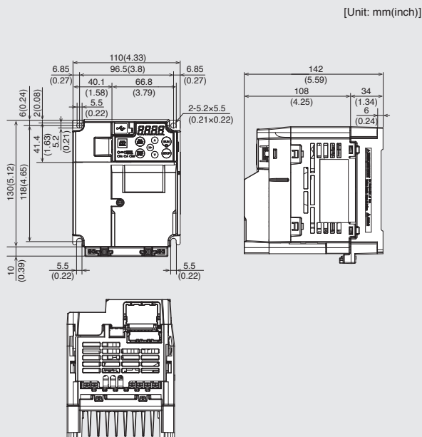
Type FRN0005E3E-7G
