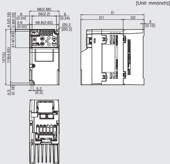
Type FRN0001E3E-7G to FRN0006E3E-7G
